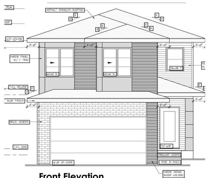
Front Elevation
